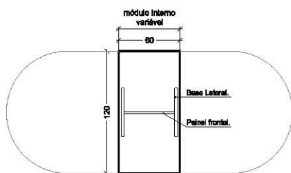
Figura 30 Mesa retangular (tampo interno retangular) MRRt 6 - 60x120cm Vista superior | Escala 1:50
